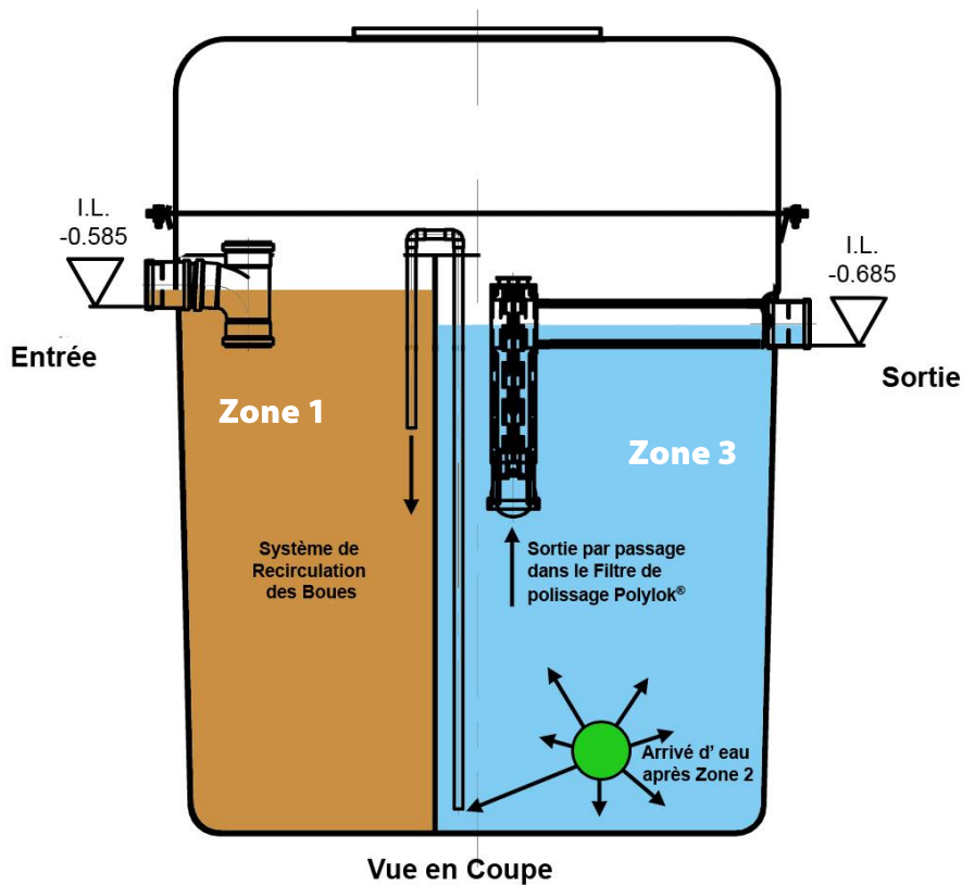
Figure #1 : Processus du Concept Epuratoire
